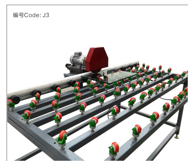
台式Low-E除膜机 Low-E Coating Removal Table Machine
