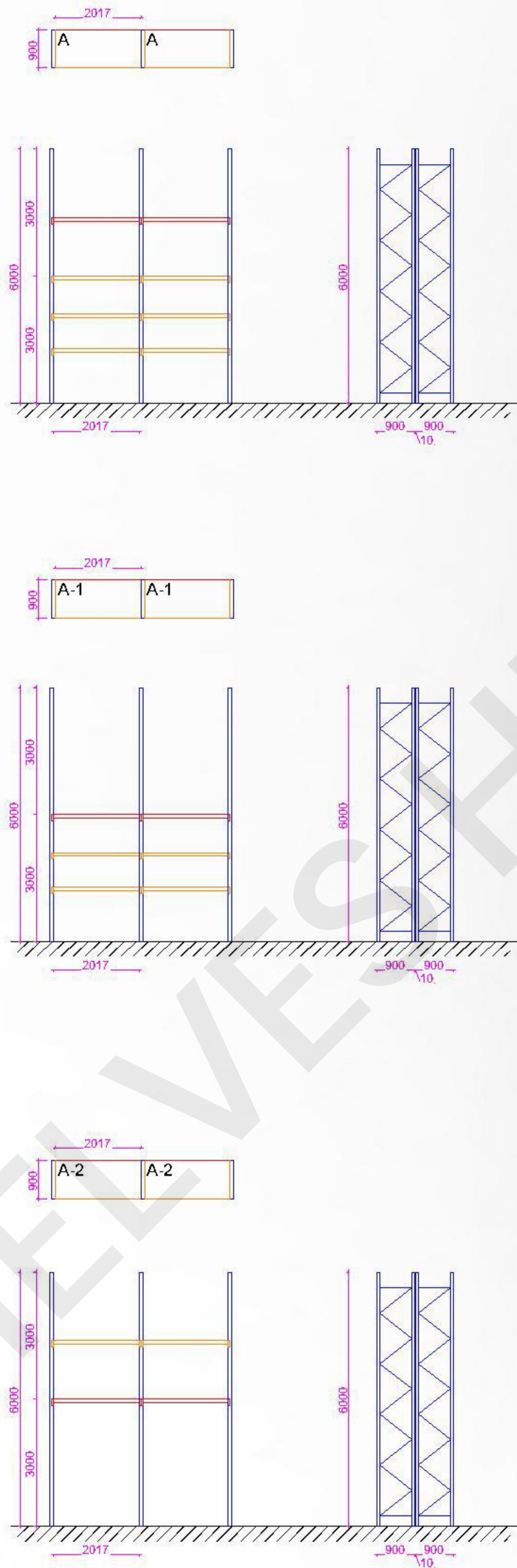
Step 2: Beam Installation drawing
