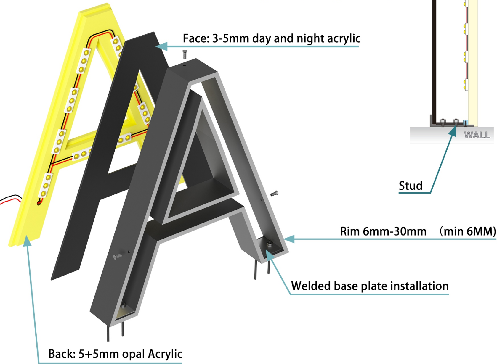
P4-11-Front & Back-lit with Black & White Panel and Acrylic Base (Standing installation)
