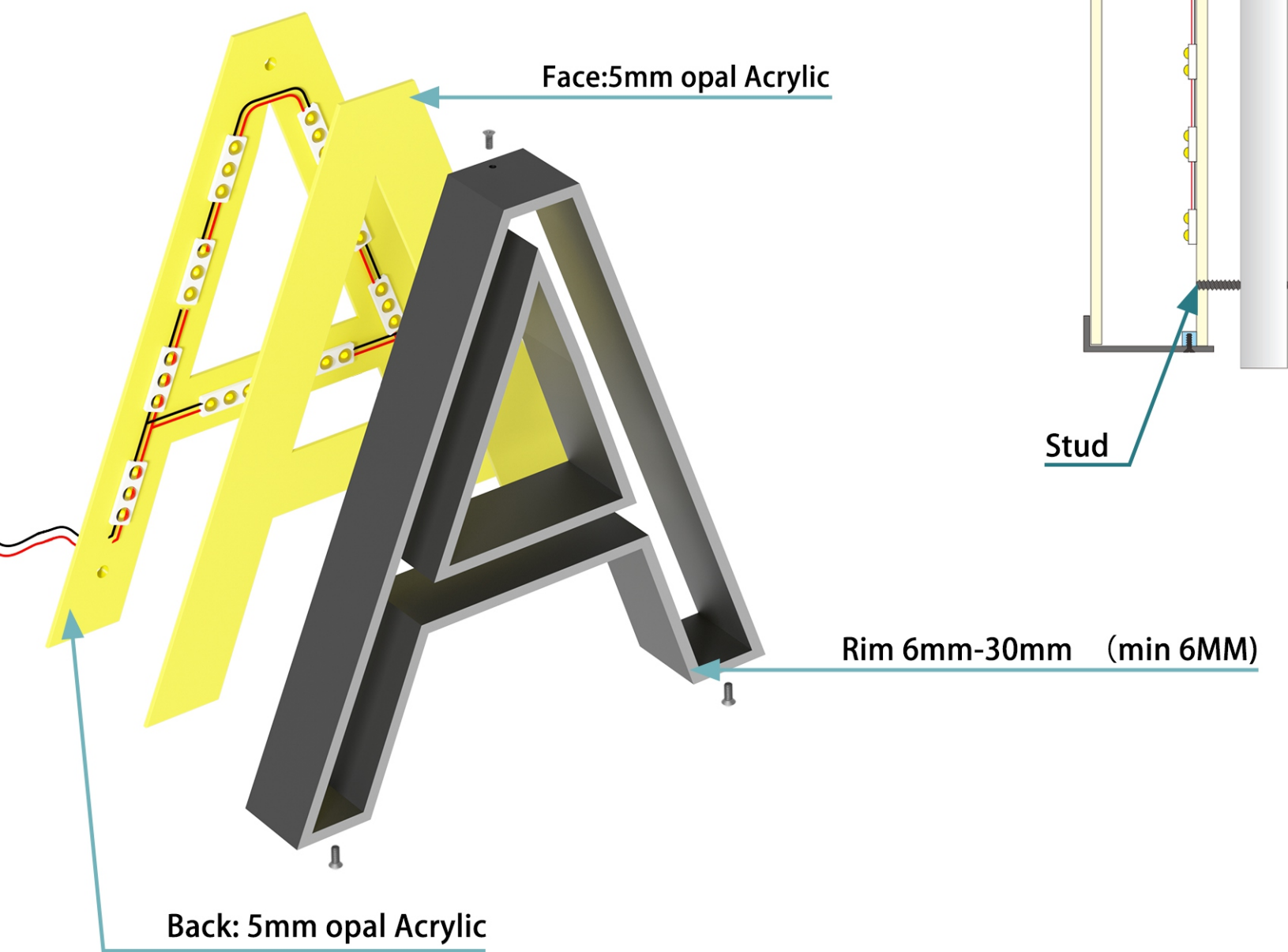
P4-4-Front & Back-lit with Acrylic Base
