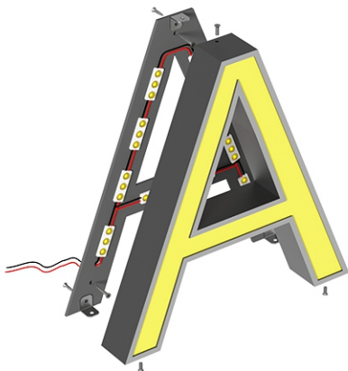
Countersunk Self-tapping Screw installed
