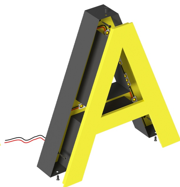
P6-2 Front and Back lighting (Acrylic not protrusion)
