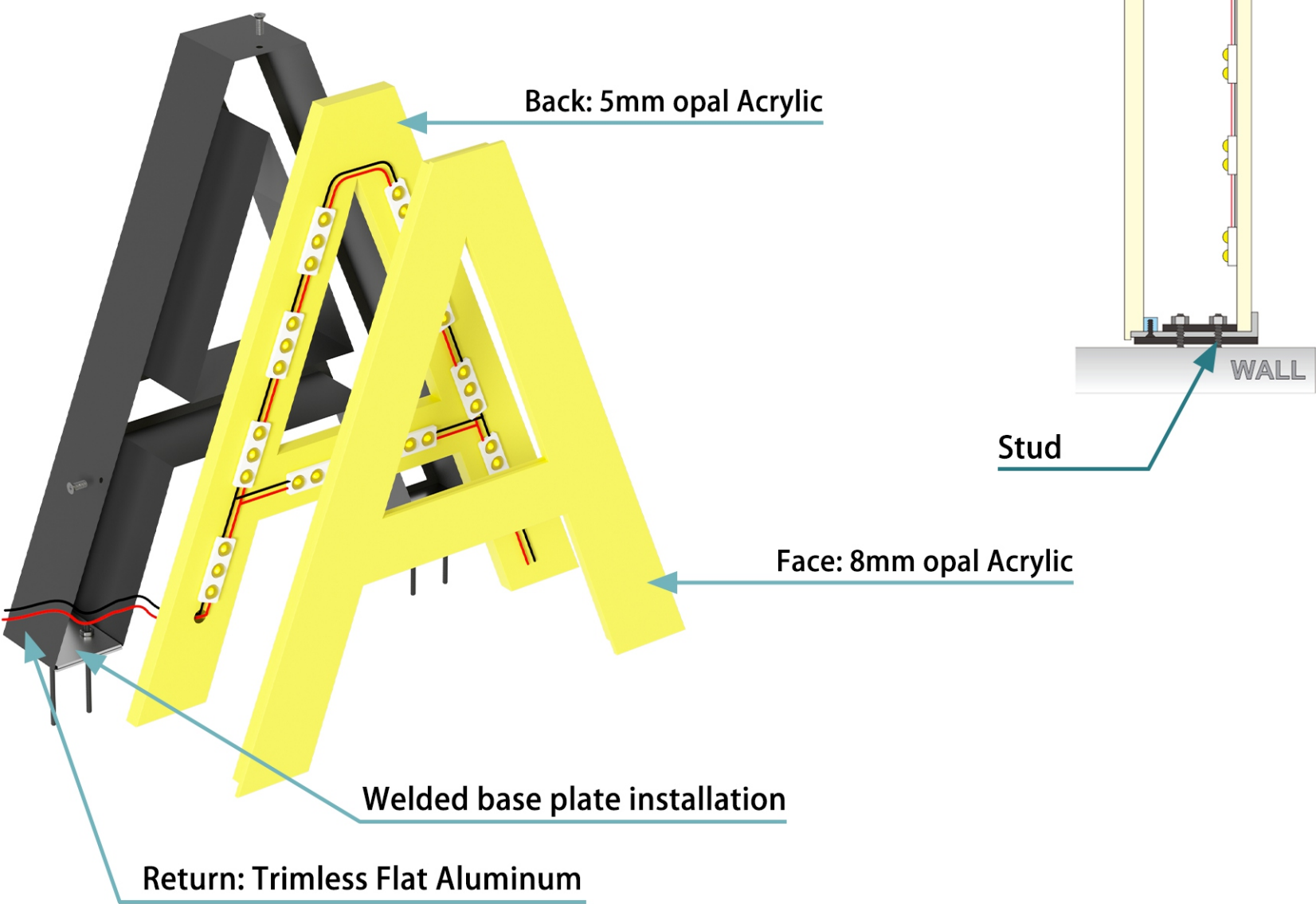
P6-4-Trimless channel Letter, Front & Back-lit (Standing installation)
