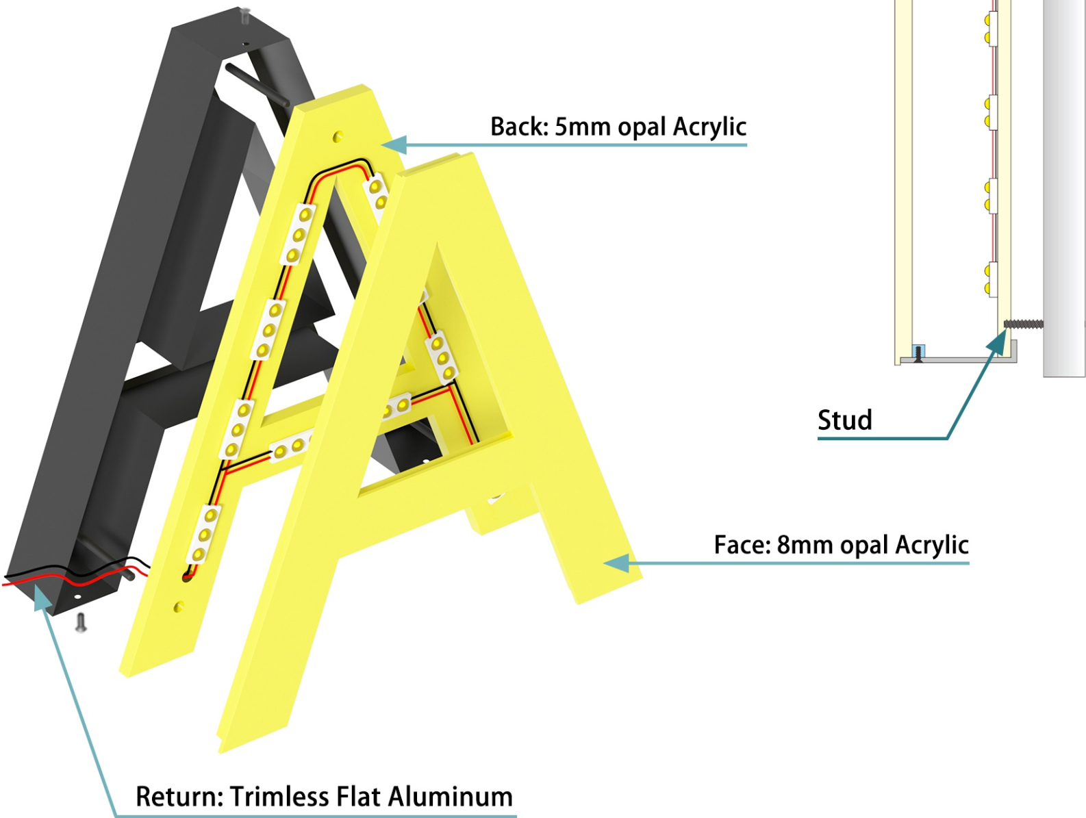
P6-1-Trimless channel Letter, Front & Back-lit
