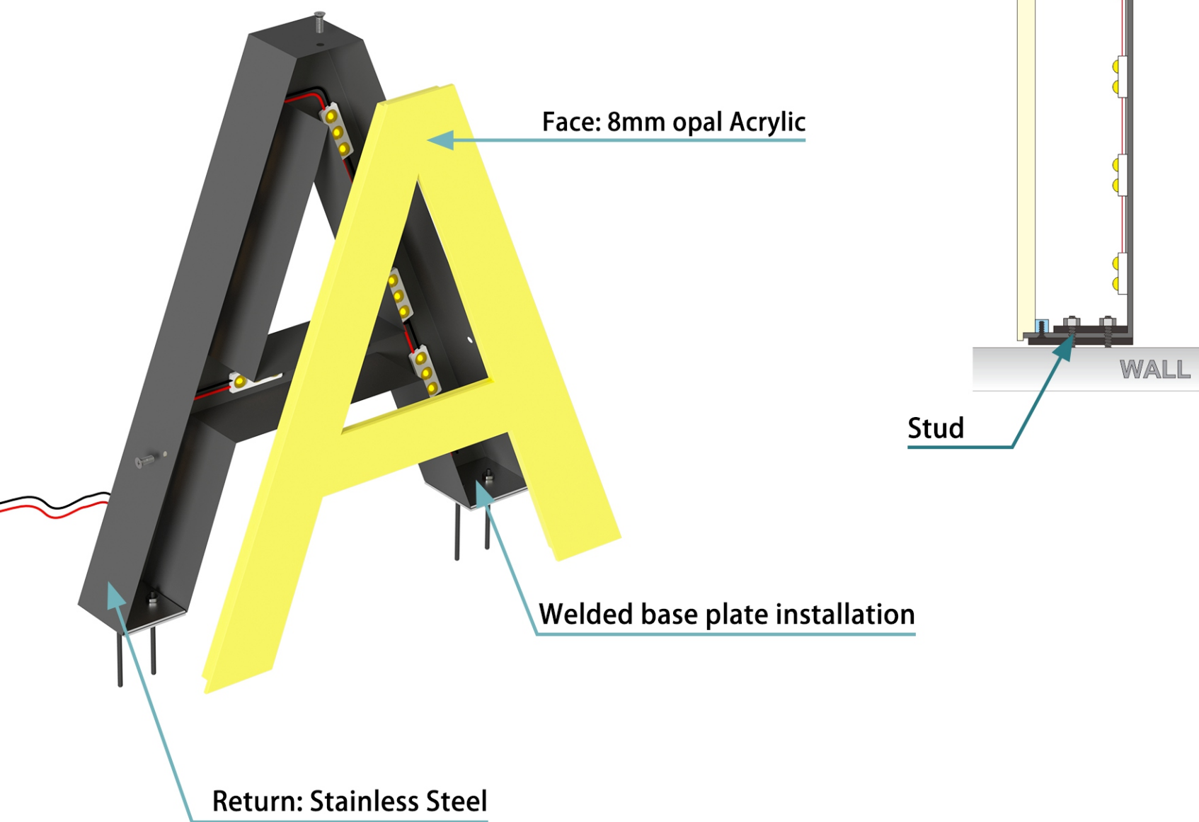
P6-6-Trimless channel Letter, Front lit (Standing installation)
