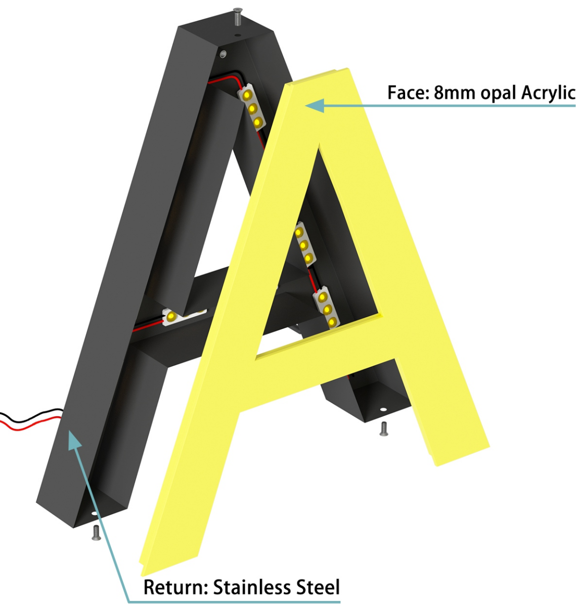
P6-3-Trimless channel Letter, Front lit
