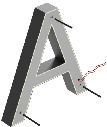
Side fixed by silicone sealant
