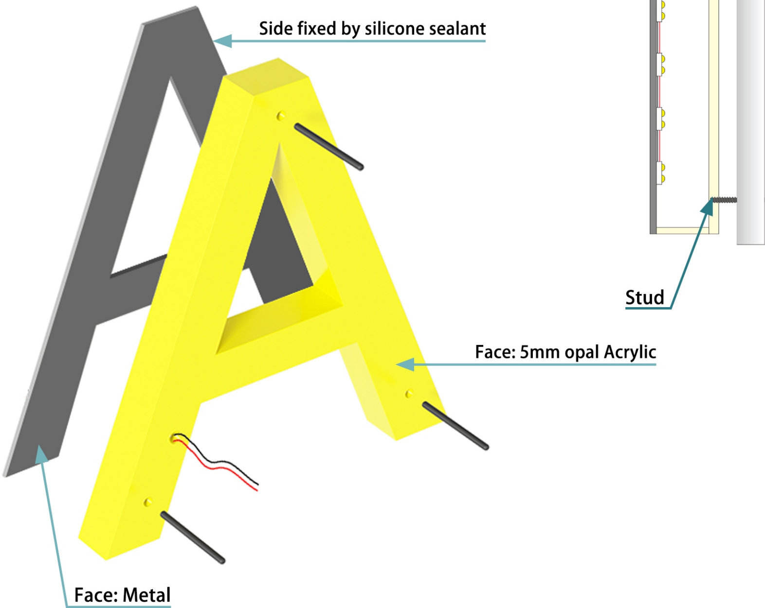
P10-2-Reverse acrylic letters side illuminated
