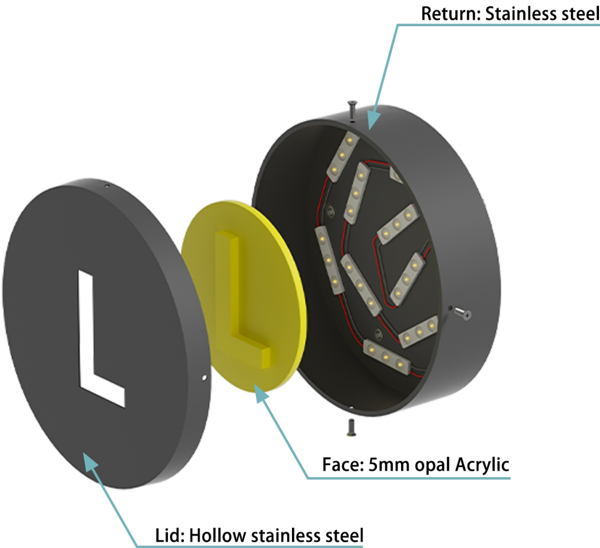
P13-8-Hollowed-Out Panel Single-Sided light box
