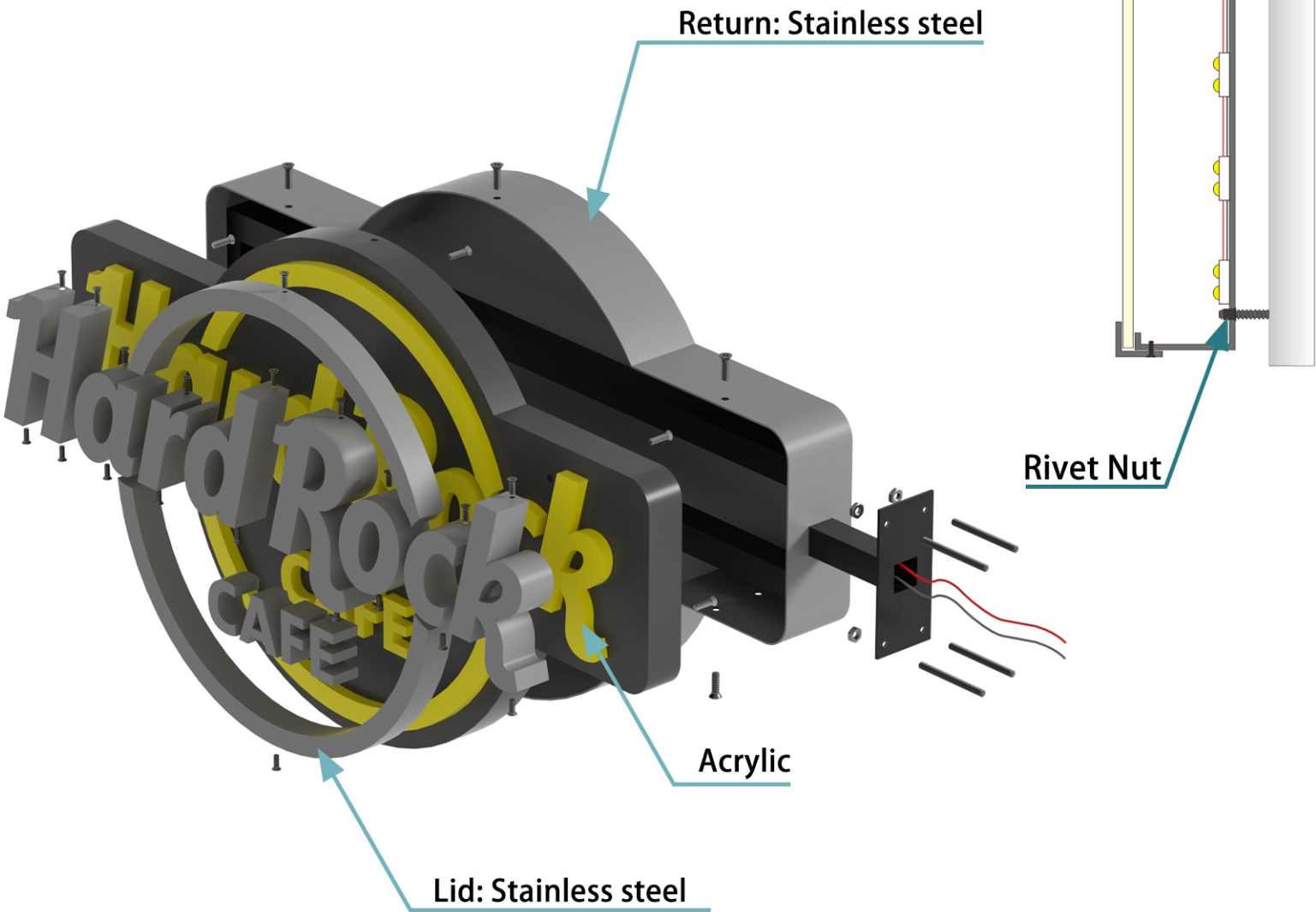
P13-11-Customized single sided light box
