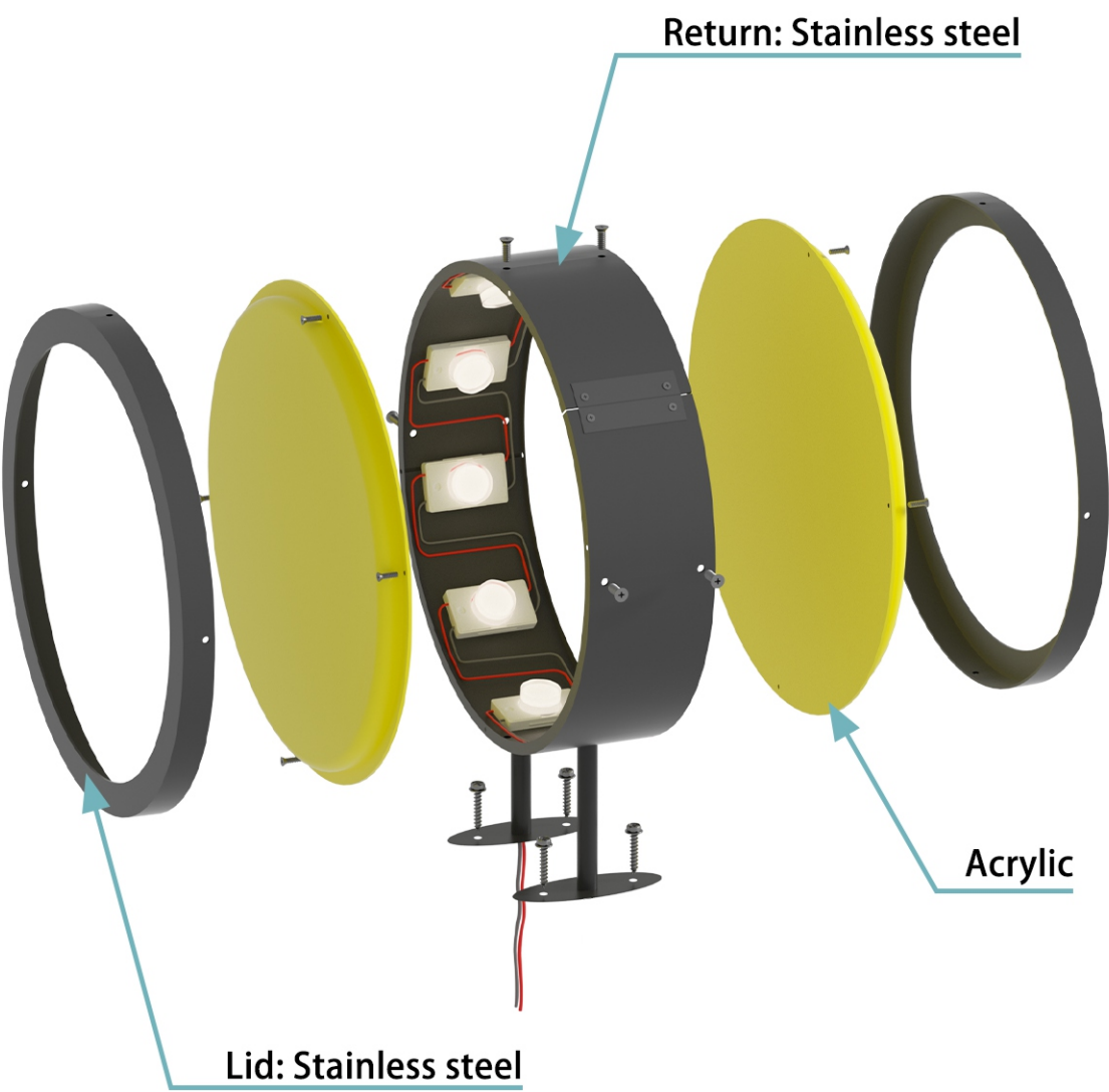
P13-17-Vacuum-Formed Double sided Light Box
