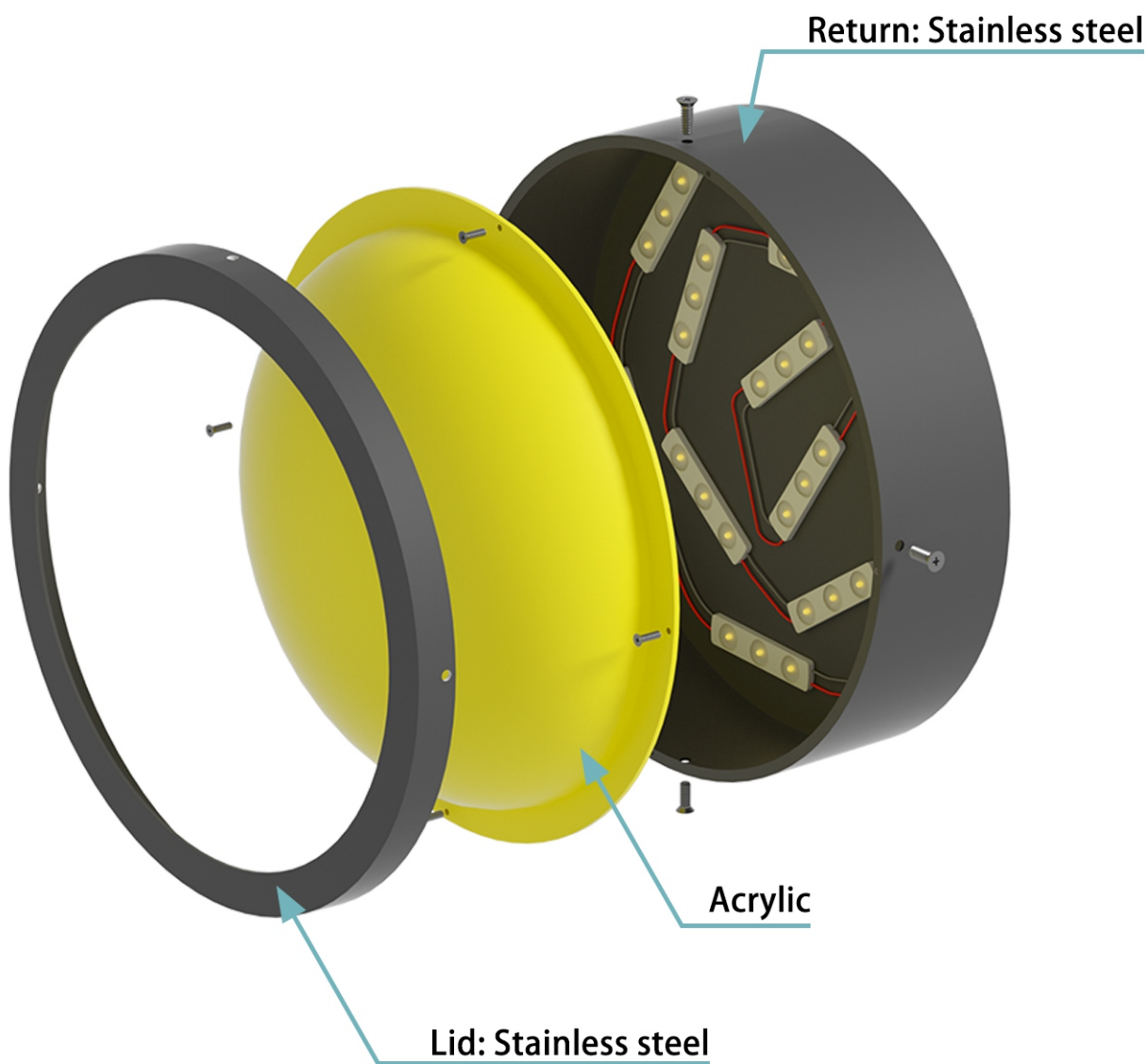
P13-16-Vacuum-Formed Single sided Light Box
