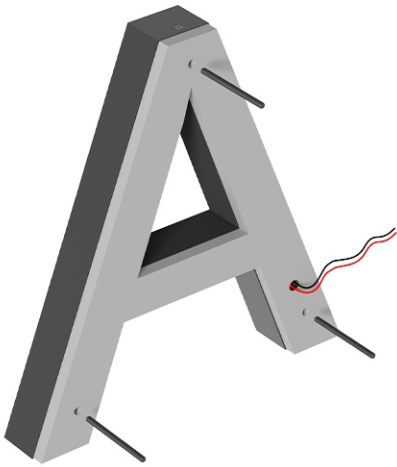
Self-tapping stud fastening
