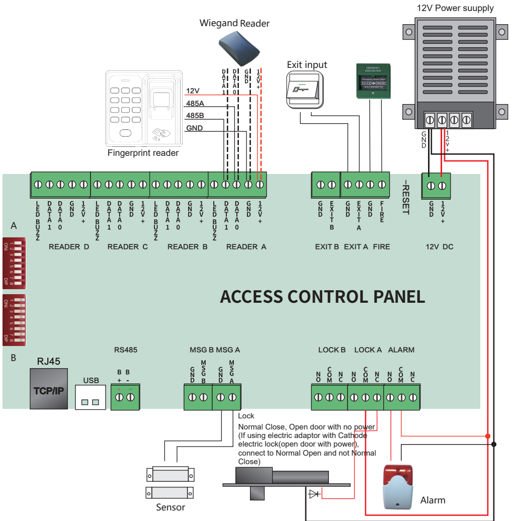
Two-Door Two-Way Wiring Diagram
