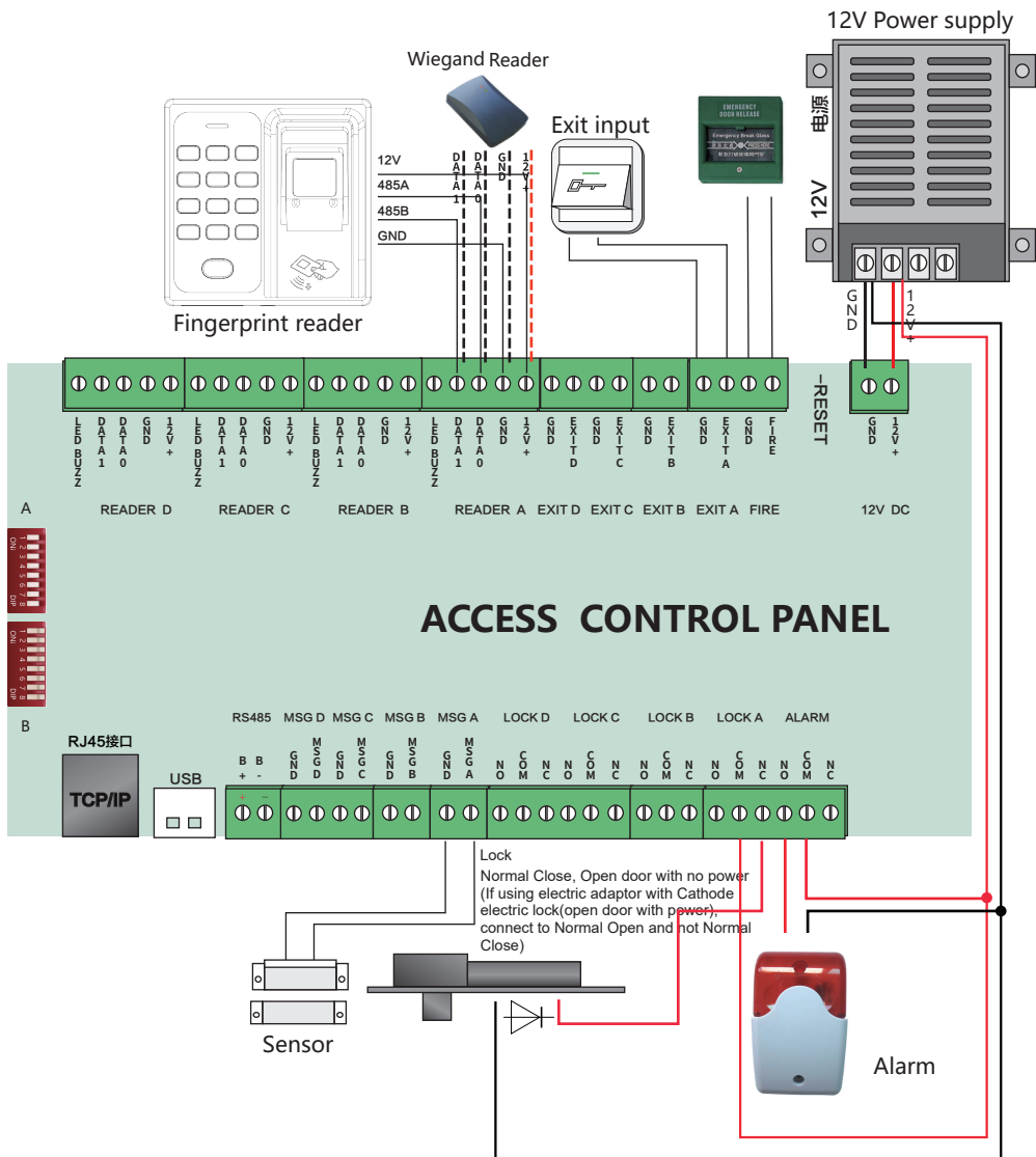
Four-Door Single-Way Wiring Diagram
