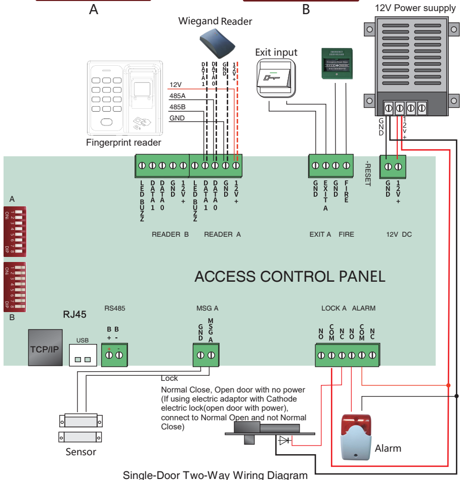
Single-Door Two-Way Wiring Diagram
