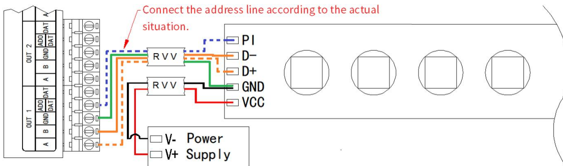
Output control TTL signal, address line write code DMX lamps and lanterns
