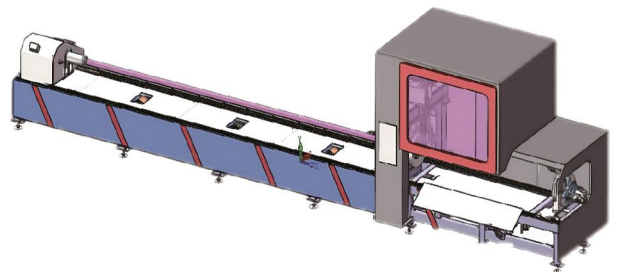
Three Chuck of Laser Pipe Cutting Machine
