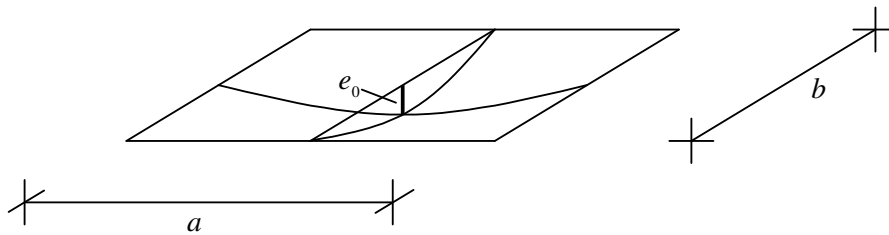
Figure 5.1: Initial equivalent geometric bow imperfection e_0 of a plate segment
